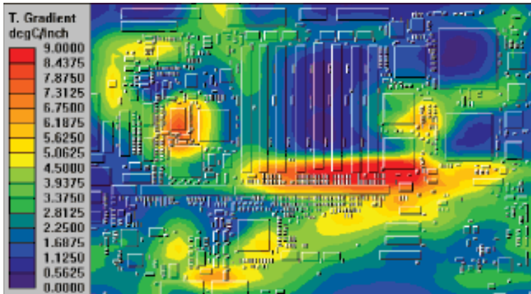
Thermal analysis is available directly from within PADS Standard Plus.
