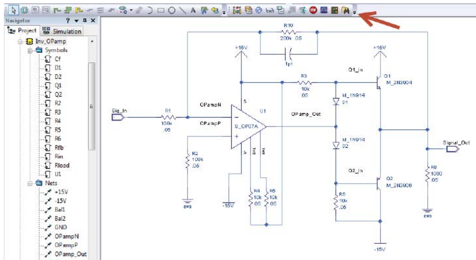
PADS Standard Plus schematic includes an integrated analog simulation environment that makes it easy to drive simulation and PCB layout and shorten overall design time.
